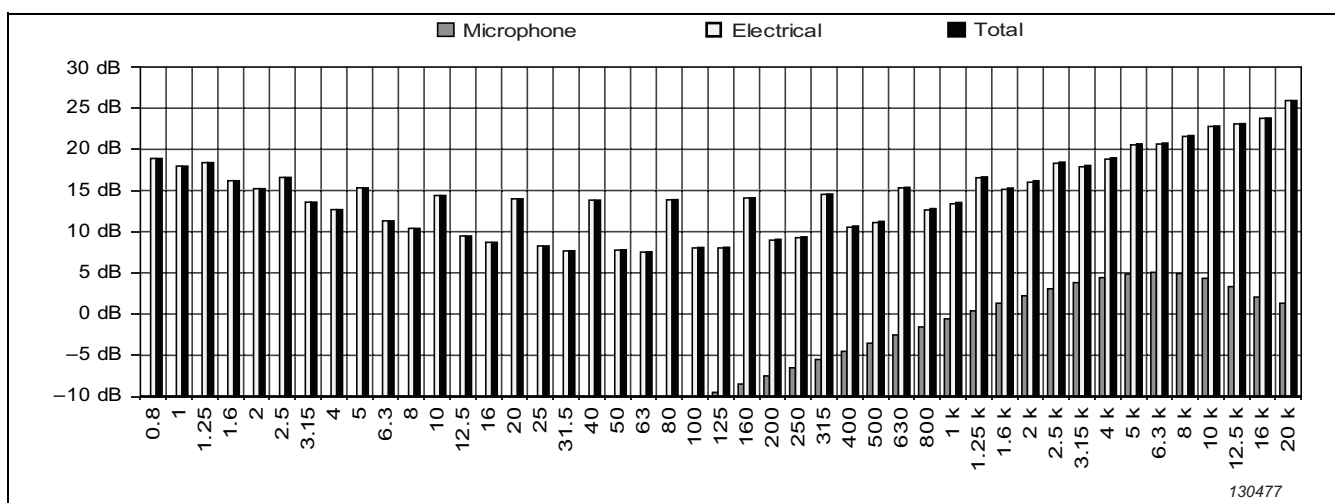
Fig. 4.29b Typical self-generated noise, 1/3-octave band, Low Range, with UC-0211
