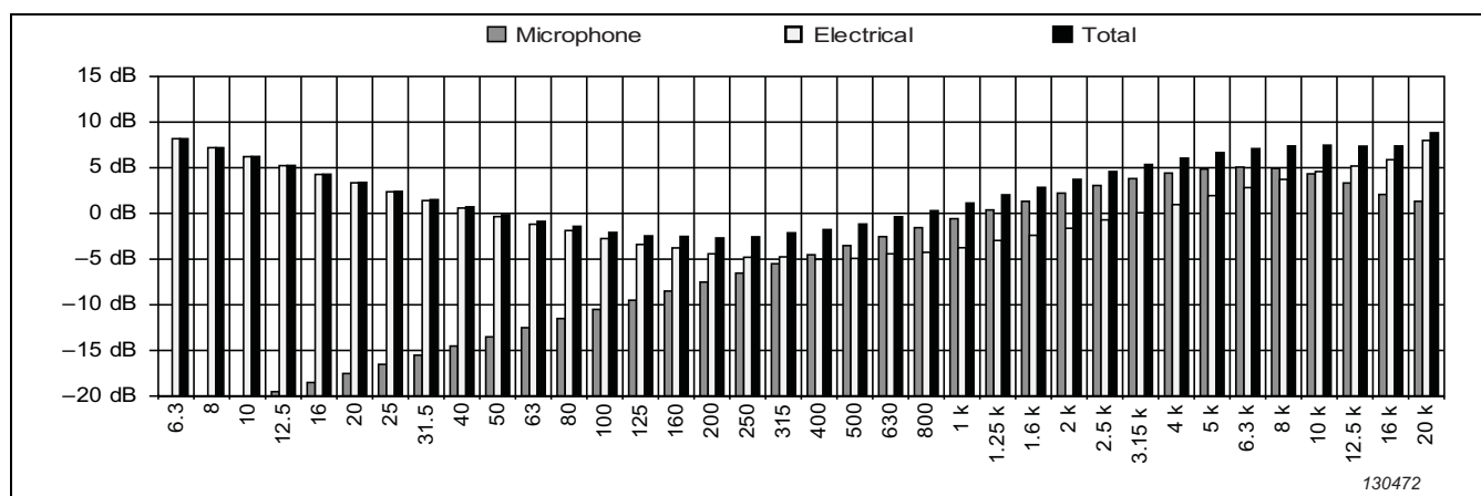
Fig. 4.27b Typical self-generated noise, 1/3-octave band, Single-range, with UC-0211
