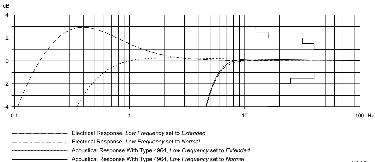
Fig.4.2b Typical low-frequency responses with UC-0211
