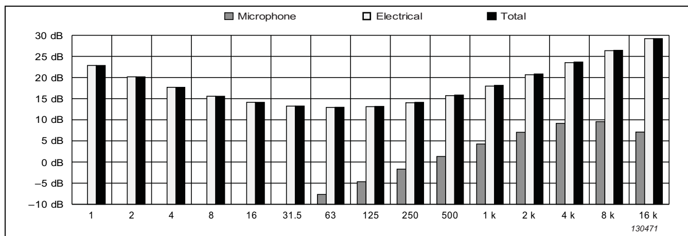
Fig. 4.27a Typical self-generated noise, 1/3-octave band, Single-range, without UC-0211
