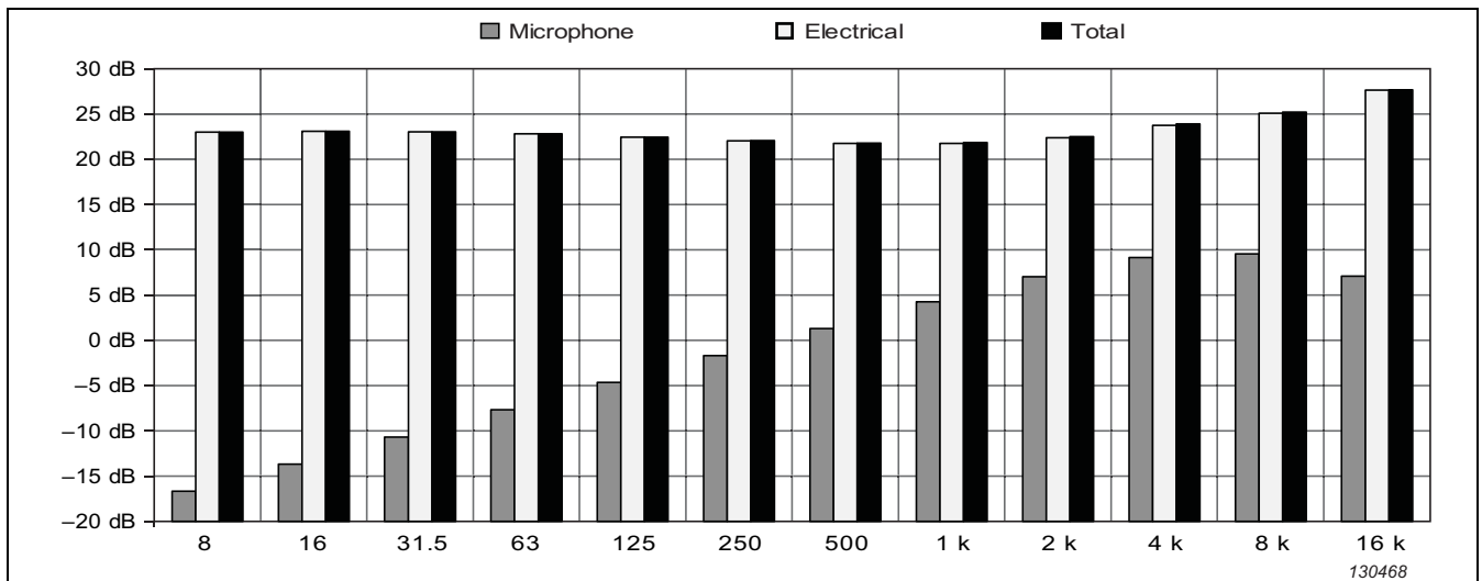
Fig.4.25b Typical self-generated noise, 1/1-octave band, High Range, with UC-0211
