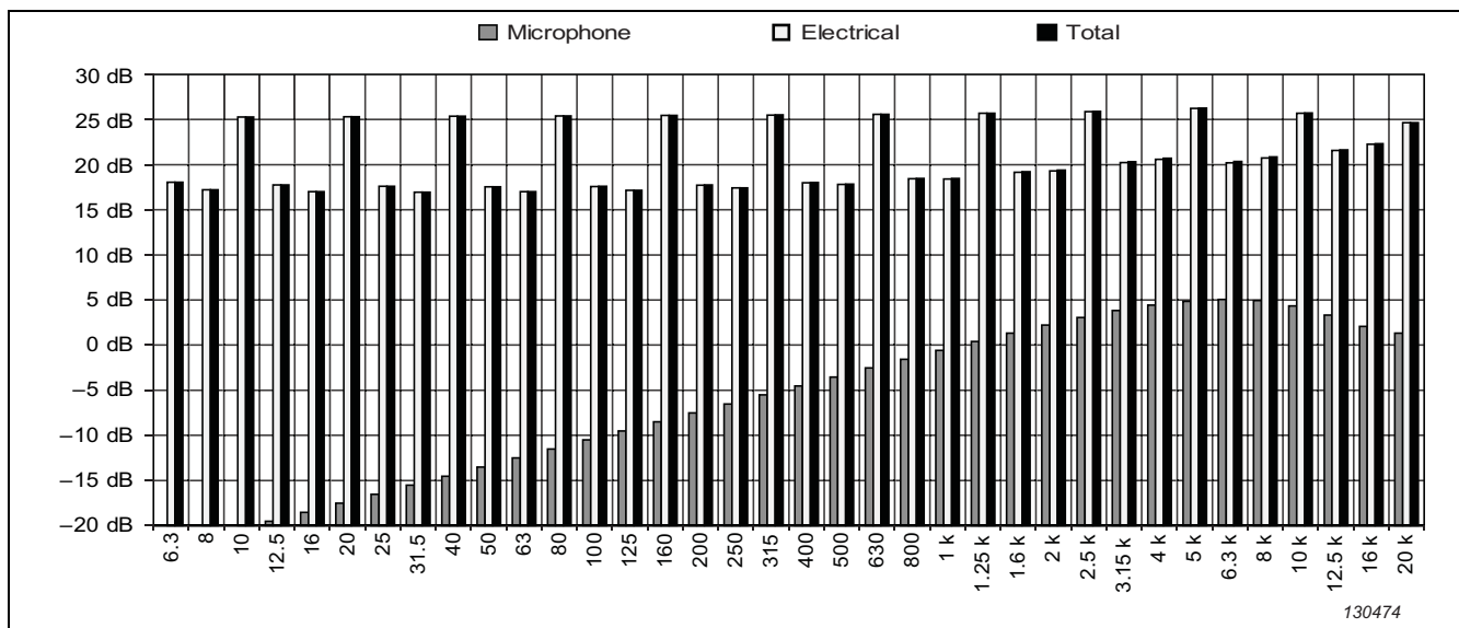
Fig.4.28b Typical self-generated noise, 1/3-octave band, High Range, with UC-0211
