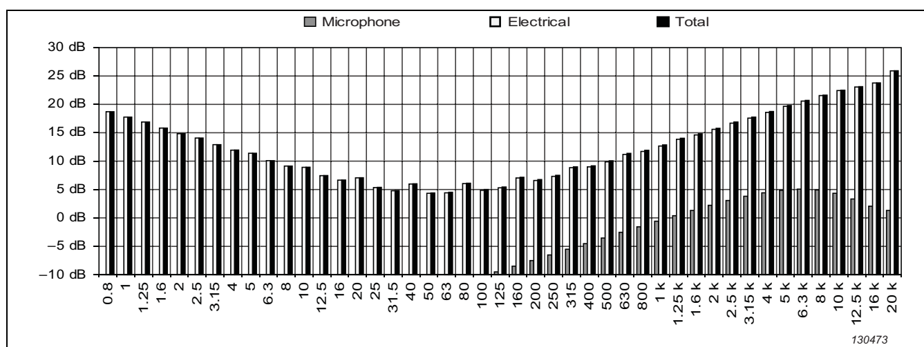
Fig. 4.27b Typical self-generated noise, 1/3-octave band, Single-range, with UC-0211
