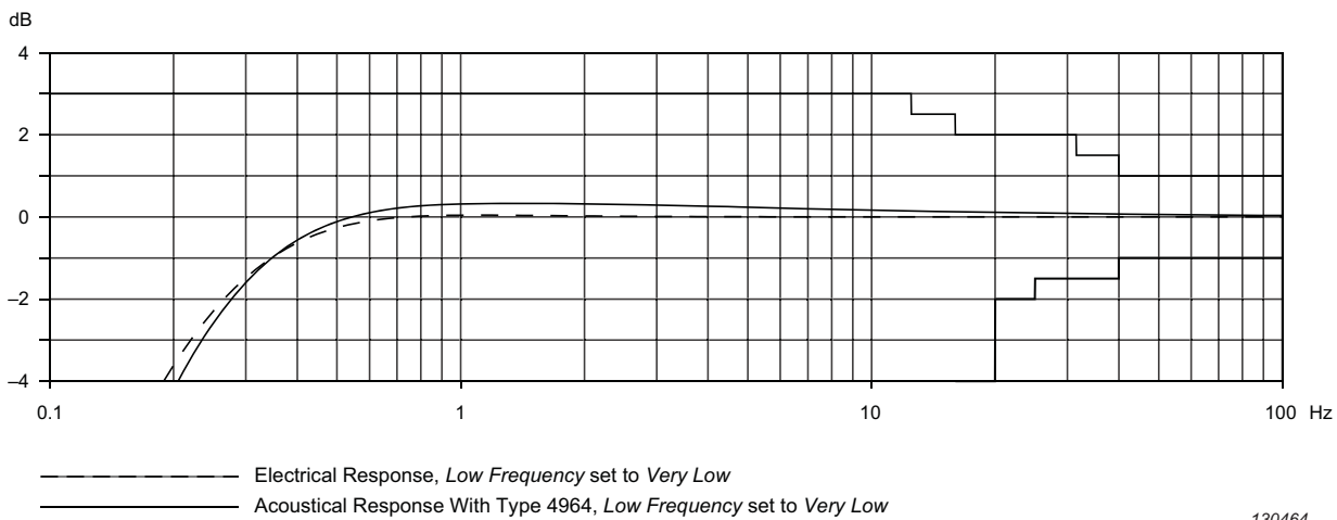
Fig.4.2b Typical low-frequency responses with UC-0211
