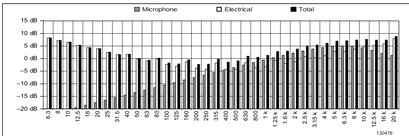
Fig. 4.29b Typical self-generated noise, 1/3-octave band, Low Range, with UC-0211
