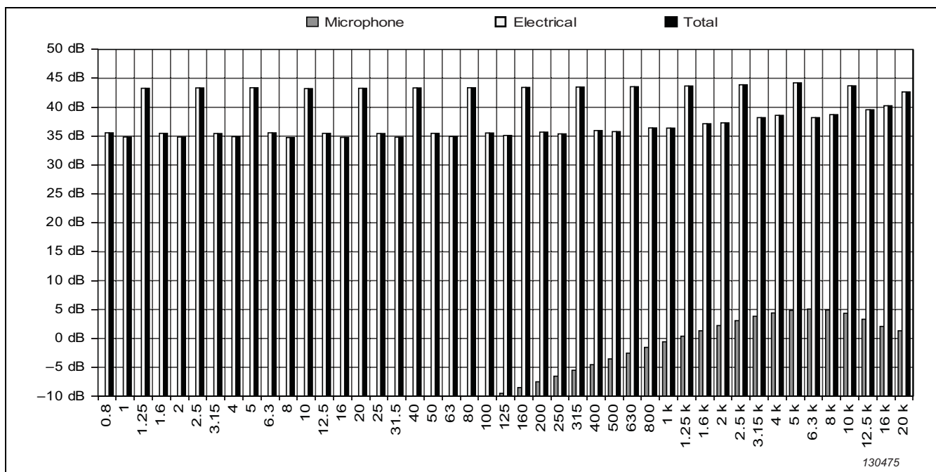
Fig.4.28b Typical self-generated noise, 1/3-octave band, High Range, with UC-0211
