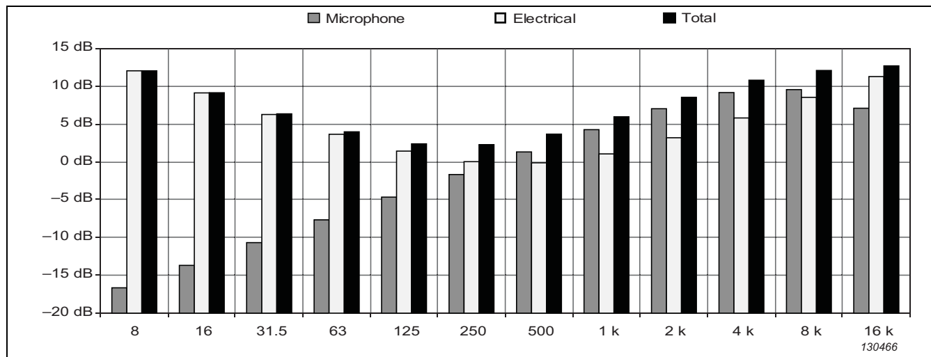
Fig.4.24b Typical self-generated noise, 1/1-octave band, Single-range, with UC-0211
