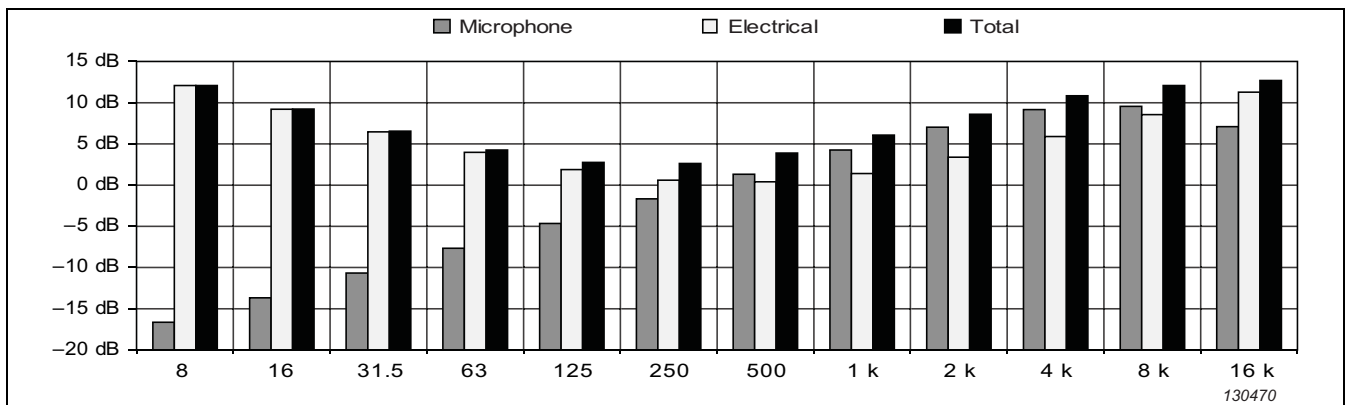
Fig.4.26a Typical self-generated noise, 1/1-octave band, Low Range, without UC-0211
