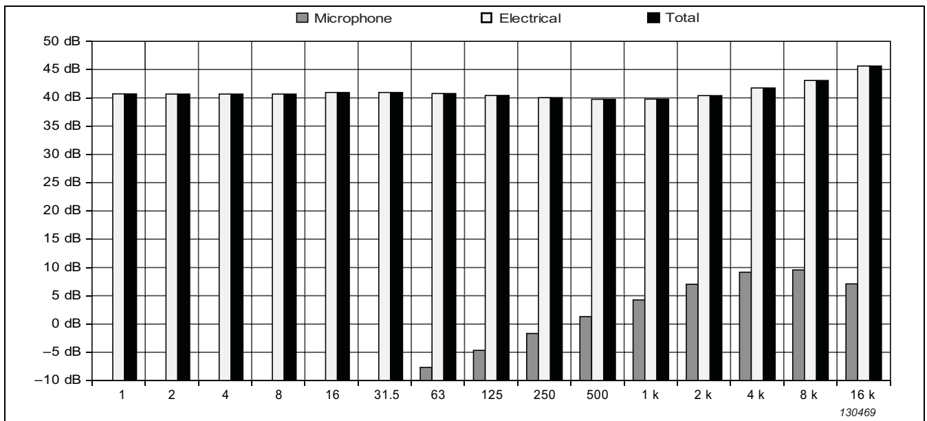
Fig.4.26a Typical self-generated noise, 1/1-octave band, Low Range, without UC-0211
